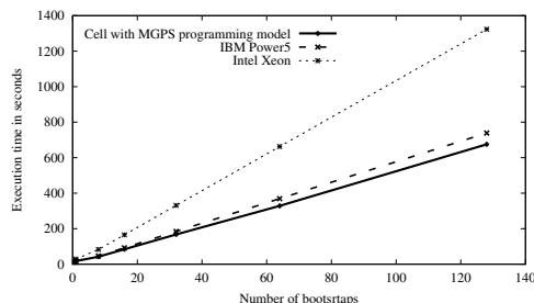
FIGURE 3: RAxML performance on different multi-threaded and multicore microprocessors: Intel Xeon, IBM Power5 and Cell. The number of ML trees created is 1, 8, 16, 32, 64 and 128.
